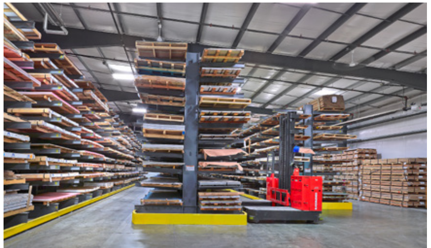
Photo: Very Narrow Aisle (VNA) Cantilever Racking
