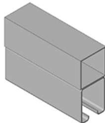
Track #2: Galvanized track welded to 2" x 2" reinforcement tube.
