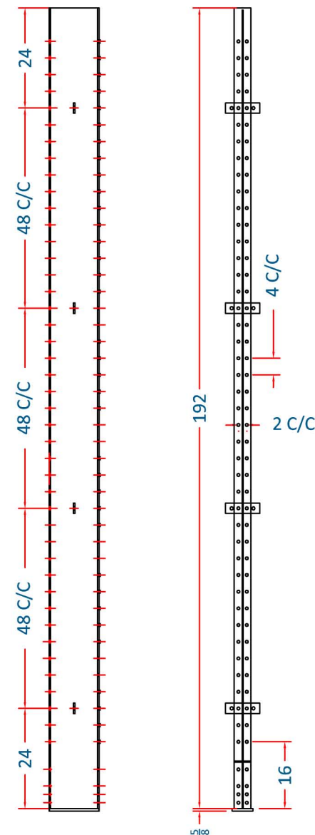
(W12x16) 16'-0" HIGH DOUBLE-SIDED COLUMN WITH A CAPACITY TO SUPPORT UP TO 8,000-LBS PER SIDE
