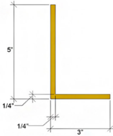
PROFILE VIEW L5" x 3" x 1/4"
